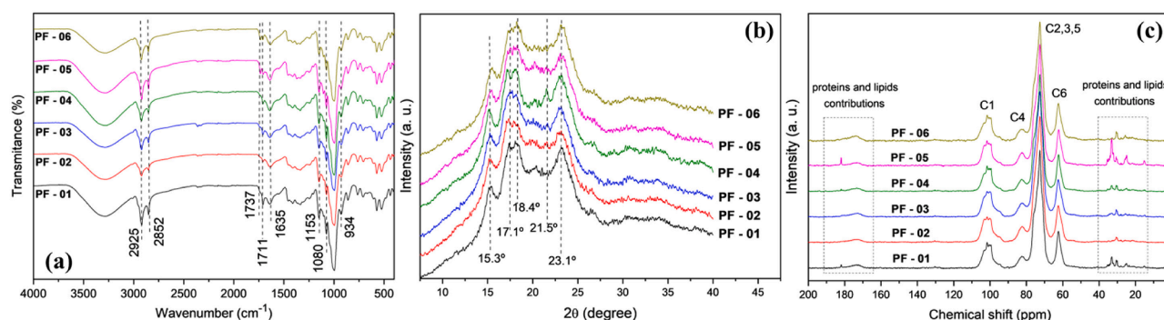
Fig. 2. (a): FTIR spectra of the six pupunha flour (PF) samples with the identification of the main vibrational bands; (b): X-ray diffractograms of the six pupunha flour (PF) samples with the identification of the main crystalline planes; (c): structural composition of the six pupunha flour (PF) samples identified by solid-state ^{13}\text{C} CPMAS spectra.
