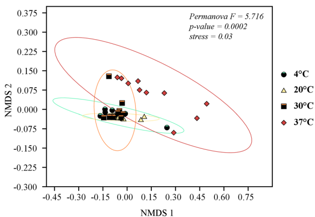
Fig. 6 Impact of temperature on the diversity of the functional profiles. Non-metric Multidimensional Scaling (NMDS) based on Bray-Curtis similarity matrix of predicted pathways for each sample at 4 (dots), 20 (triangle), 30 (square), and 37 °C (diamond). Groups are surrounded by ellipses (95% Confidence interval around centroid). Permutational analysis of variance (PERMANOVA) F and p values are displayed at the top right of NMDS plot
