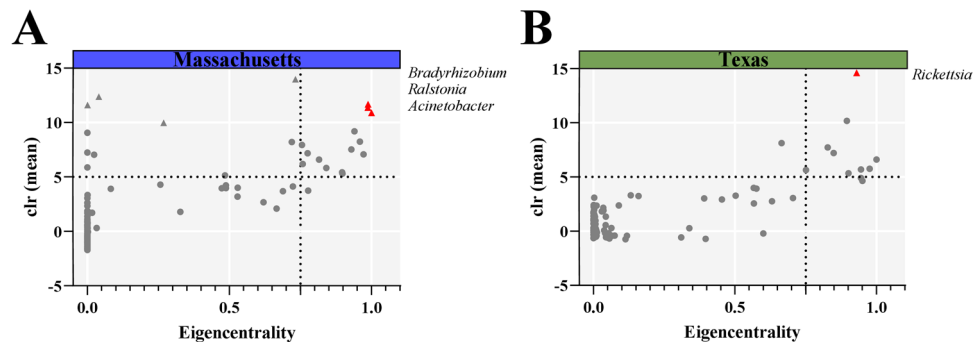
Fig. 8 Keystone taxa in field-collected ticks. Scatter plot showing the mean relative abundance (expressed as clr) and the eigencentrality of each bacterial taxon (dots or triangle) of the microbial community from I. scapularis collected from Massachusetts (A) and Texas (B). The red dots or triangle represent bacterial taxa that are present across all the samples of I. scapularis collected from different loca-
