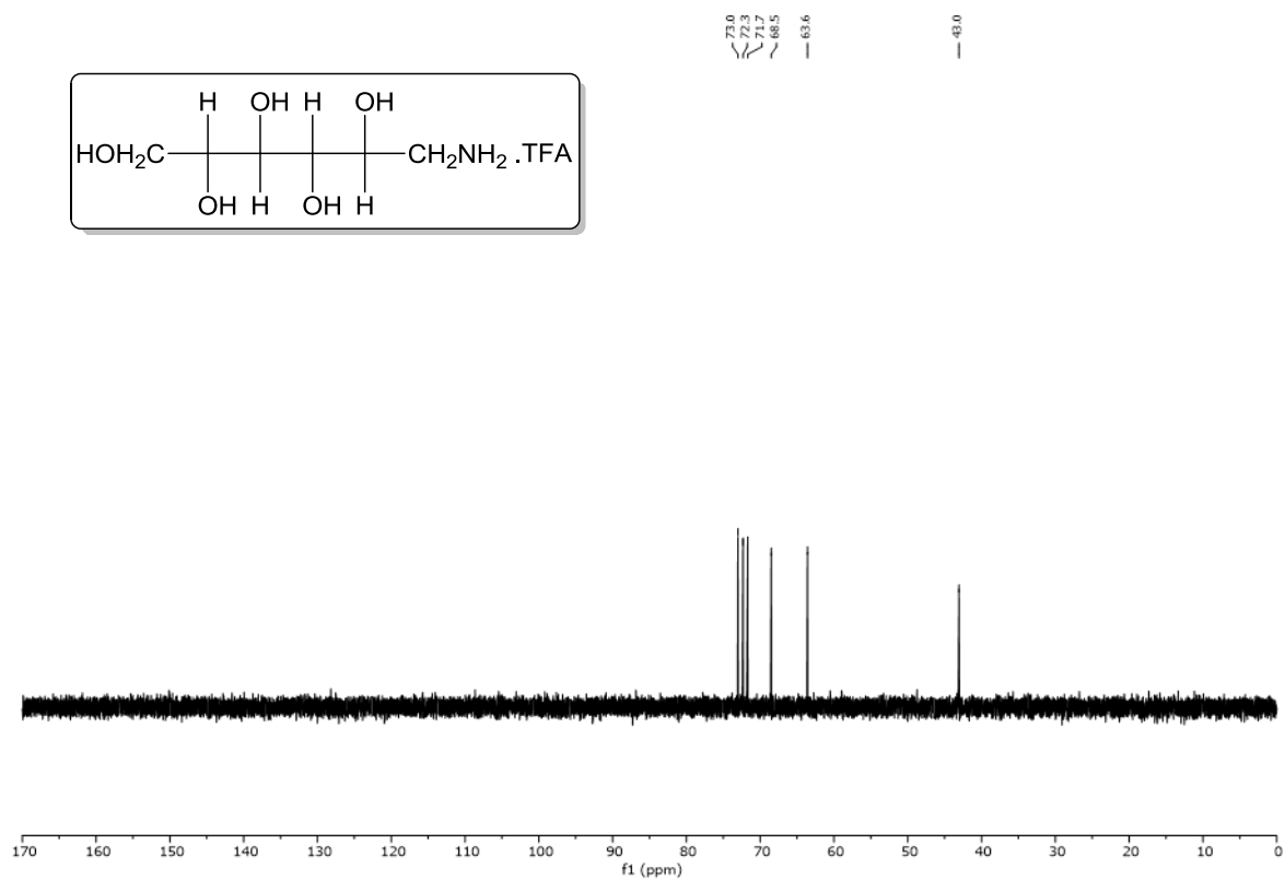
Figure S9: 13 C NMR spectrum of iditolamine in D 2 O.
