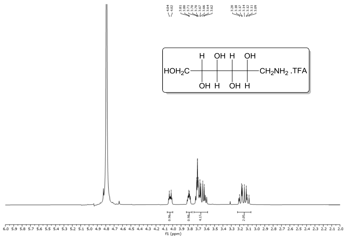
Figure S8. 1 H NMR spectrum of iditolamine in D 2 O.
