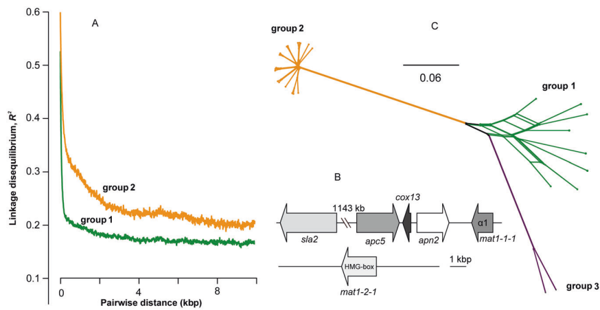
Fig. 2 Analysis of the recombination pattern in the L. rhizalophila population. A Linkage disequilibrium (LD) decay between pairs of SNPs, measured as R^2 , with distance on the same scaffold. B Mating structure and organization of L. rhizalophila JP-R-44 suggested its homothallic reproduction mode. sla2 : cytoskeleton assembly control protein, (protein ID 13068); apn2 : DNA lyase (protein ID 13428);
