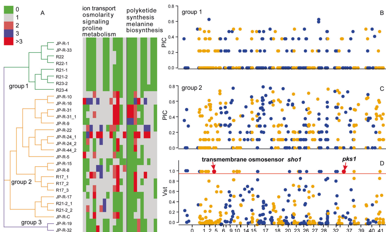
Fig. 3 Genome-wide copy number variation profiles across the 29 L. rhizohalophila individuals. Loci encompassing salinity-responsive and melanin-biosynthetic genes with highly differentiated copy numbers between L. rhizohalophila groups are outlined. A Loci encompassing salinity-responsive and melanin-biosynthetic genes with highly differentiated copy numbers between L. rhizohalophila groups are outlined. B , C , D PIC and Vst values (y-axis) calculated with overlapping 10-kbp windows across all the contigs (x-axis) are plotted. The horizontal red line represents Vst values of 1.
