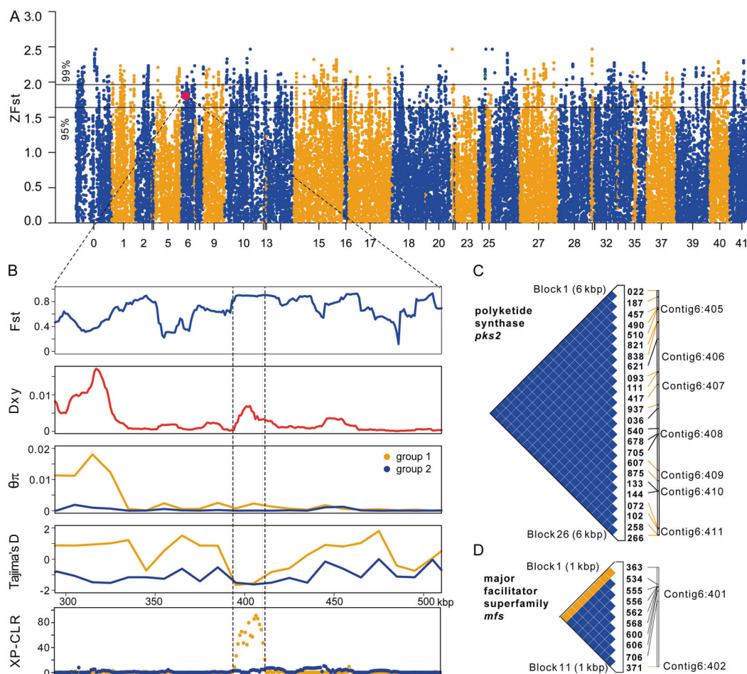
Fig. 4 Genetic differentiation and detection of positive selection signals in the L. rhizohalophila population. A Genome-wide distribution of the Z-transformed fixation index ZFst plotted along contigs between group 1 and group 2. Scaffolds are arranged on the x-axis according to the reference genome and are separated by color. Genes within every 10-kbp window are plotted in a single column, and the 95% and 99% outliers are marked. B Enlargement of a genomic island of divergence (containing six genes) in scaffold 6, in which a strong positive selection signal in group 1 is detected. The genomic region
