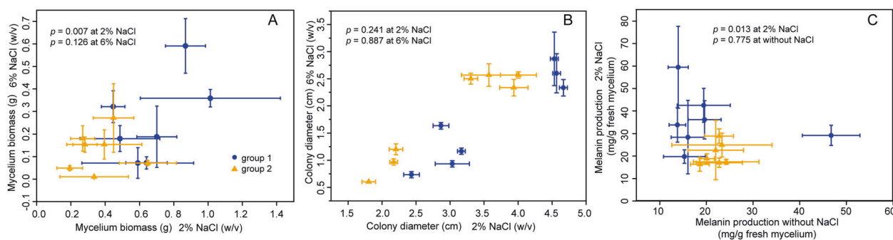
Fig. 5 Melanin synthesis and mycelial growth of representative isolates from group 1 and group 2. For measurement of colony diameter and biomass, 2% and 6% NaCl levels were used. A Biomass comparison between the two groups under salinity stress conditions. B Growth rate on the PDA plates added with 2% and 6% NaCl. C Comparison of melanin production between the two groups
