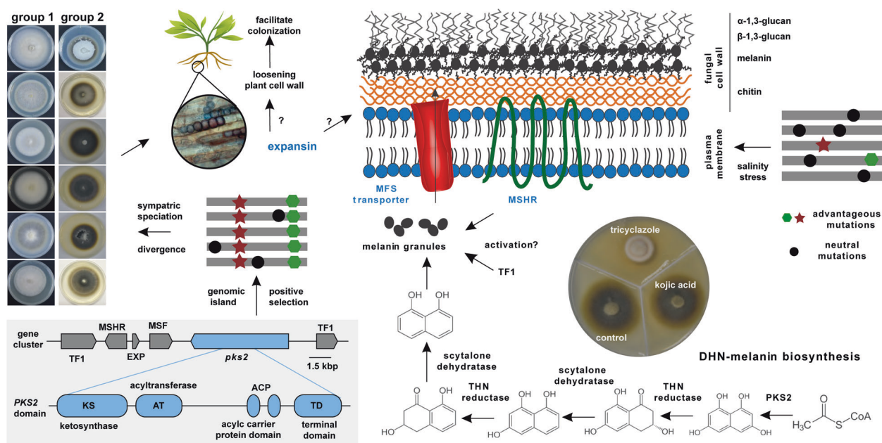
Fig. 6 A schematic outline showing the potential effect of positive selection on the melanin biosynthetic gene cluster in L. rhizohalophila . PKS2 catalyzes the first step of melanin biosynthesis. The use of melanin biosynthesis inhibitors (tricyclazole and kojic acid, 50 \mu\text{g mL}^{-1} ) confirmed that L. rhizohalophila synthesized dihydroxynaphthalene melanin (DHN-melanin), as colonies growing in the presence of kojic acid, the inhibitor of dihydroxyphenylalanine (DOPA) melanin, appeared normal and were indistinguishable from the controls. The representative isolates from group 1 and group 2 grown on PDA without NaCl for two weeks at 25^\circ\text{C} are shown.
