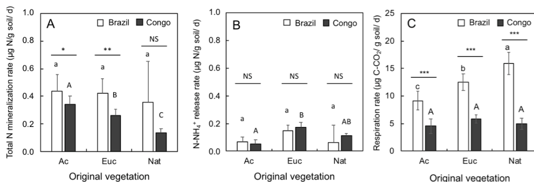
Figure 1. Rates of total nitrogen mineralization ( \text{N-NH}_4^+ + \text{N-NO}_3^- ) (A), \text{N-NH}_4^+ production (B), and respiration (C) measured in soil samples taken from topsoil (0–20 cm) under different vegetation of origin: Acacia (Ac), Eucalyptus (Euc), and native vegetation (Nat) in Brazil (Itatinga, white bars) and Congo (Kissoko, dark grey bars). Each bar represents mean ( n = 9 ) with a confidence interval ( p = 0.05 ). Different letters on bars (lowercase for Brazil and uppercase for Congo) indicate significant differences among original vegetation (one-way ANOVA and Tukey's HSD post hoc test at p \leq 0.05 ). Asterisks indicate site effects (Student's t -test): NS ( p > 0.05 ), * ( p < 0.05 ), ** ( p < 0.01 ), *** ( p < 0.001 ).
