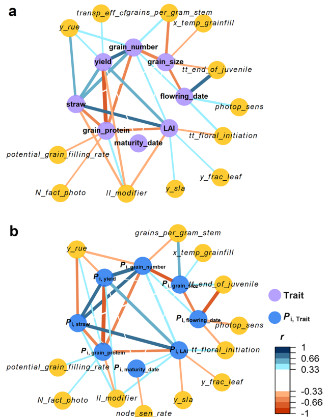
Fig. 6 r -network between 90 physiological parameters, P_{i, trait} (a) and traits (b) of randomly selected 1000 virtual genotypes ( SPG=1 ) grown under 9000 environments ( SPE=1 ). Node (circle) represents mean trait (purple), P_{i, yield} (blue) or physiological parameters (yellow). Description of physiological parameters: number of grains that are set depending on the stem dry weight ( grain\_per\_gram\_stem ), efficiency of roots to extract soil water ( ll\_modifier ), rate of node senescence on main stem ( node\_sen\_rate ), multiplier for nitrogen deficit effect on photosynthesis ( N\_fact\_photo ), potential rate of grain growth at grain filling ( potential\_grain\_filling\_rate ), sensitivity to photoperiod ( photop\_sens ), transpiration efficient ( transp\_eff\_cf ), thermal time between plant emergence and end of juvenile stage ( tt\_end\_of\_juvenile ), thermal time between end of juvenile and floral initiation ( tt\_floral\_initiation ), temperature affecting stress index for the potential grain filling rate ( x\_temp\_grain\_fill ), fraction of dry matter allocated to rachis for specific stages ( y\_frac\_leaf ), radiation use efficiency ( y\_rue ), potential leaf specific area ( y\_sla ) (colour figure online)
