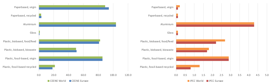
FIGURE 3 Comparison of (left) CEENE values in MJex/kg of material and (right) IPCC values in kg CO 2 eq/kg for raw materials originating from Europe or world regions ( source: Ecoinvent database v3.5).
