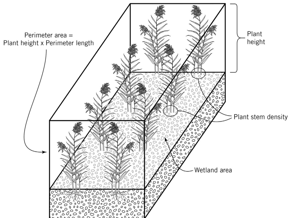
Fig. 3. Illustration of perimeter area (perimeter length \times plant height) relative to wetland area.
