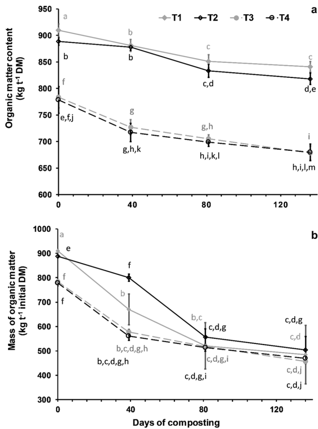
Fig. 4 Dynamics of (a) the content and (b) mass of organic matter during composting: T1-dry palm leaves, T2-dry palm leaves and rock phosphate, T3-dry palm leaves and sheep manure, and T4-dry palm leaves, sheep manure, and rock phosphate. Letters indicate significant differences ( p < 0.05 ) between windrows
