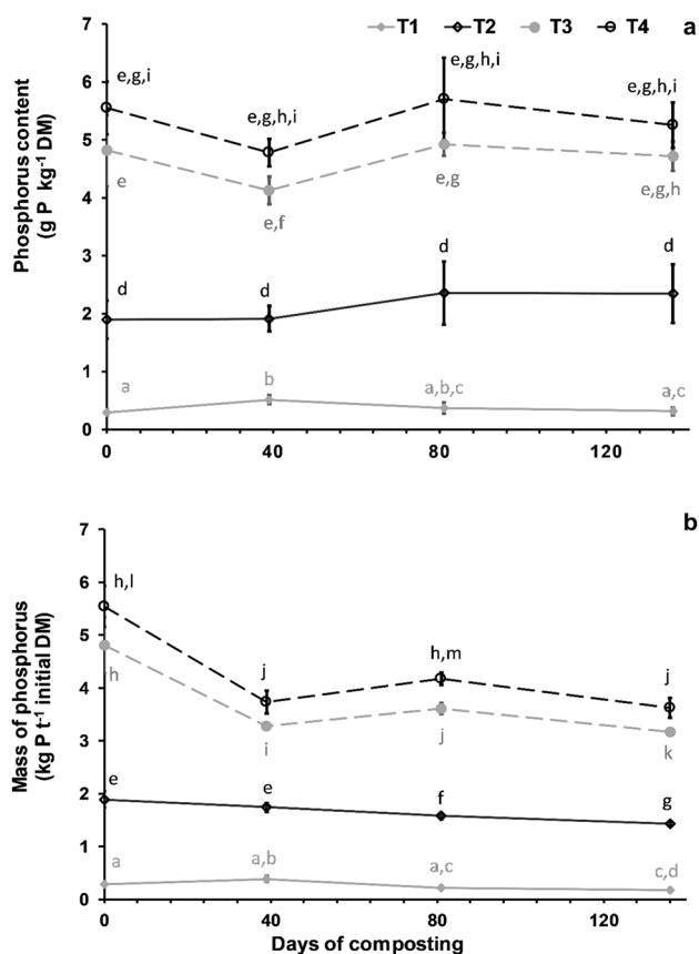
Fig. 6 Dynamics of (a) the content and (b) mass of phosphorus during composting: T1-dry palm leaves, T2-dry palm leaves and rock phosphate, T3-dry palm leaves and sheep manure, and T4-dry palm leaves, sheep manure, and rock phosphate. Letters indicate significant differences ( p < 0.05 ) between windrows
