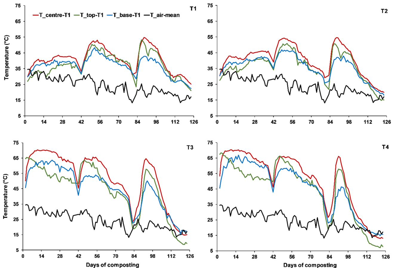
Fig. 3 Temperature dynamics during composting (for all treatments). T1-dry palm leaves, T2-dry palm leaves and rock phosphate, T3-dry palm leaves and sheep manure, and T4-dry palm leaves, sheep manure, and rock phosphate
