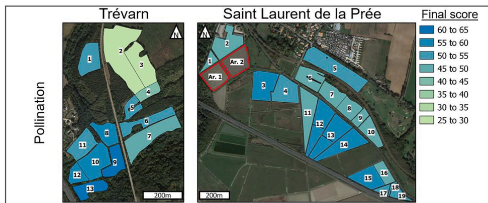
Fig. 6. Mapped final impact scores of individual permanent grassland fields on the two case-study farms for pollination. Ar. 1 and Ar. 2 represent an arable field converted into two grassland fields in a strategy proposed to optimise the provision of ES.
