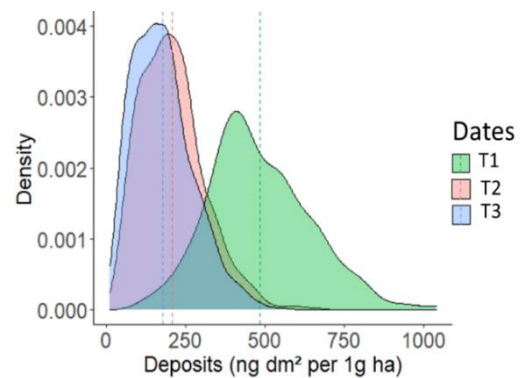
Figure 1. Empirical density curves of deposition values as a function of spray date (T1, T2, T3) obtained from calibration data. (The dashed lines indicate the mean value of the deposits observed for each date).
