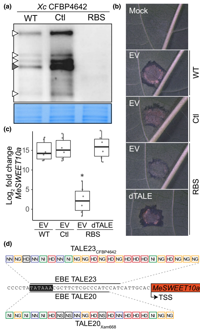
Fig. 4 Nonvascular pathogen Xanthomonas cassavae ( Xc ) relies on tal e genes for full virulence on cassava ( Manihot esculenta ) and for the induction of the expression of MeSWEET10a sugar transporter gene. (a) Western blot analysis of Xc total protein extracts resolved by SDS-PAGE using anti-TALE antibodies. Wild-type (WT) Xc CFBP4642 strain and their CRISPRi derivatives (Control -Ctl- and ribosome-binding site (RBS)) were analyzed. The upper panel shows luminescent signals (anti-TALE) in the western blot assay, while the lower panel shows protein loading by Coomassie blue staining. White arrowheads point to TALE bands; gray arrowheads point to bands with two TALEs with similar theoretical molecular weights (Supporting Information Fig. S7e). (b) Representative photographs of water-soaking symptoms observed at 5 d postinoculation on leaves of cassava cultivar CM6438-14 infiltrated with Xc CFBP4642 WT and CRISPRi derivatives transformed with pME6010-empty vector (EV) or pME6010-dTALE-SW10A (dTALE). The whole experiment was repeated three times with similar results (Fig. S8). (c) Relative expression of MeSWEET10a in cassava cultivar CM6438-14 leaves at 50 h postinoculation with the WT and the complemented CRISPRi strains. Data from two replicates of the experimental set ( n = 6 ) were analyzed through a linear mixed model. Asterisks indicate significant differences to the WT-EV treatment (Tukey's test: \alpha = 0.05 ). Points over the boxplots represent individual observations. The line across the box indicates the median, while upper and lower edges indicate the 25 th and 75 th percentiles. Whiskers are extended to show the minimum and maximum values. Complete one-to-one post hoc comparisons for (c) are shown in Supporting Information Fig. S9(g). (d) Schematic representation of the predicted evolutionary convergence of Xc TALE23 CFBP4642 and Xanthomonas phaseoli pv manihotis TAL20 Xam668 . Both TALEs are predicted to bind overlapping effector-binding elements (EBEs) in the promoter sequence of MeSWEET10a ( Manes.06123400 ). The black-highlighted motif shows a putative TATA box. The red box represents the predicted transcript and TSS stands for transcriptional start site. TALEs are depicted as a string of color-coded boxes that reflect the repeat variable di-residue (RVD) sequences of each effector.
