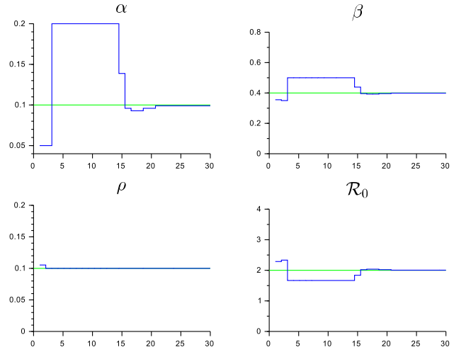
Fig. 3. Application of the alternative method on perfect data (without noise).
