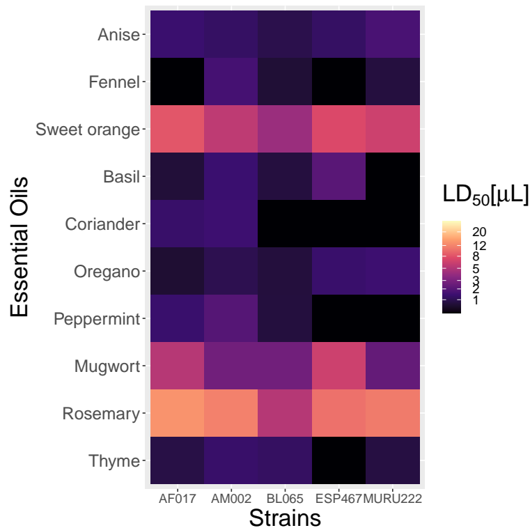
Figure 5 – Predicted LD_{50} according to the different strains (columns) and essential oils (rows). Global LD_{50} is the dose of EO at which 50% of the parasitized eggs do not emerge as adult parasitoids. Dark squares represent low LD_{50} , meaning highly toxicity of a given essential oil for a given strain.
