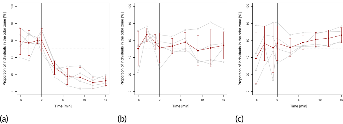
Figure 9 – Proportion of individuals in the zone with odor during the experiment: (a) Coriander essential oil and MURU222 strain; (b) Sweet orange essential oil and AM002 strain; (c) Fennel essential oil and ESP467 strain. The black vertical bar represents the introduction of odor. Dashed line symbolize the random distribution (50% individuals). The four replicates are represented by the grey broken lines and summarized by their mean and standard deviation with the dark red broken lines and error bars.
