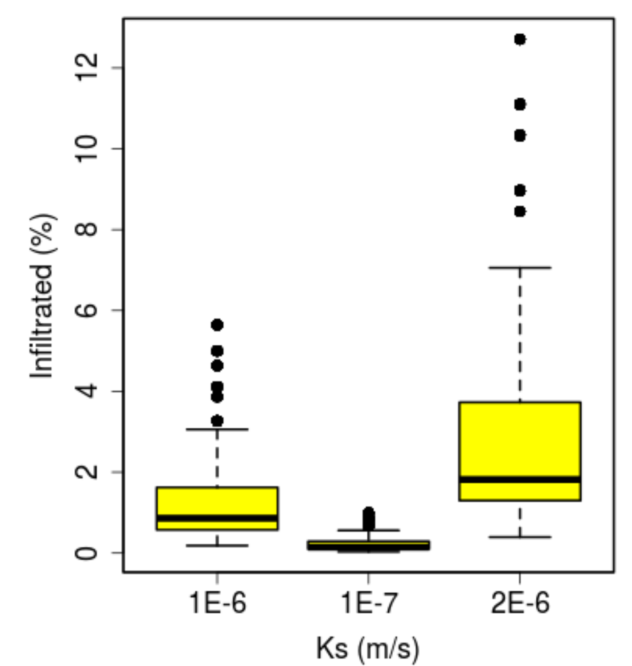
fig 6. Minor effect of infiltration on ditch retention
