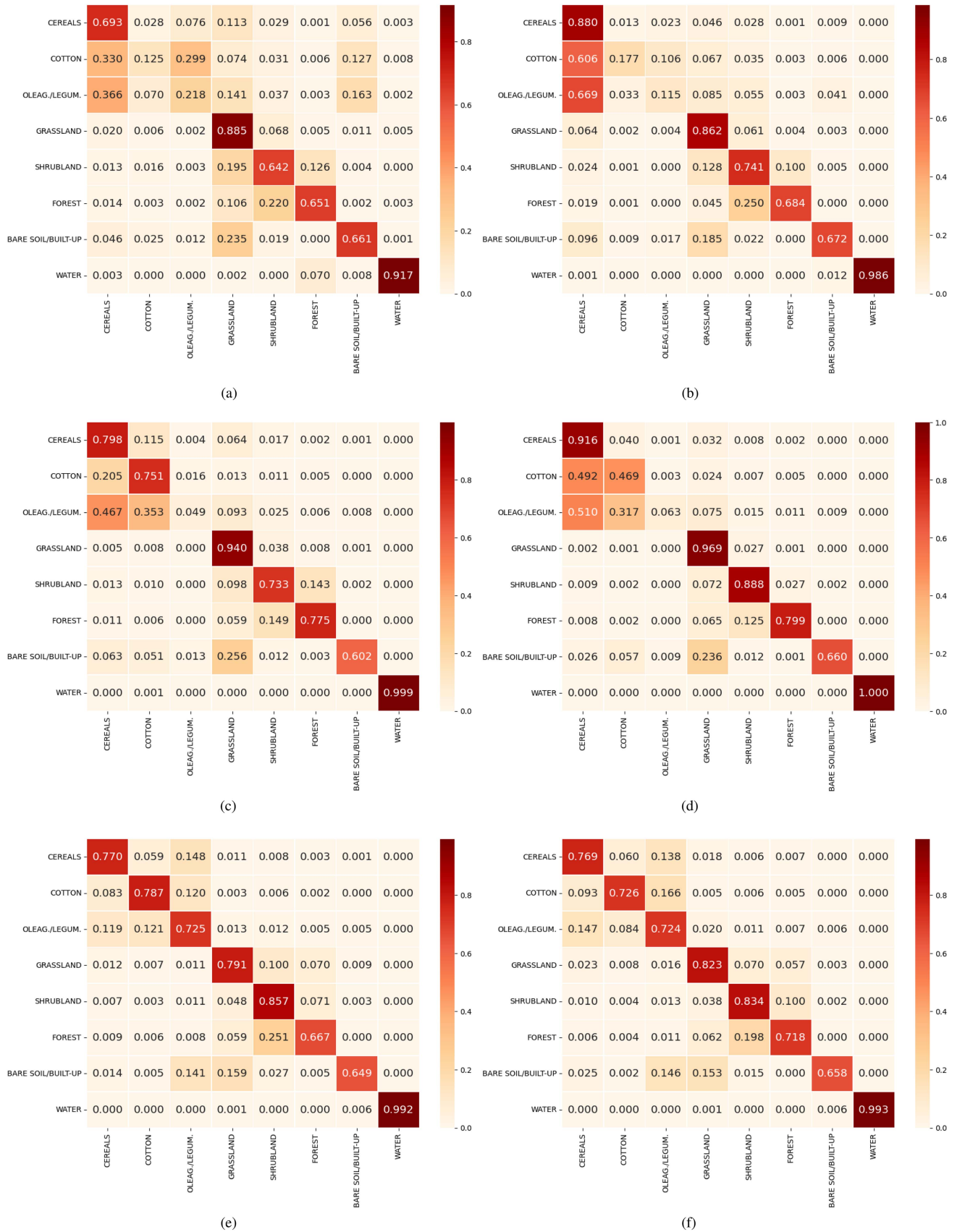
Fig. 10. Confusion matrices of the land-cover classification for the transfer task (2018 \rightarrow 2020); True class (rows) and Predicted class (columns). (a) (ONLY D_s ) TempCNN. (b) (ONLY D_s ) RF. (c) DANN. (d) SpADANN . (e) (ONLY D_t ) TempCNN. (f) (ONLY D_t ) RF.
