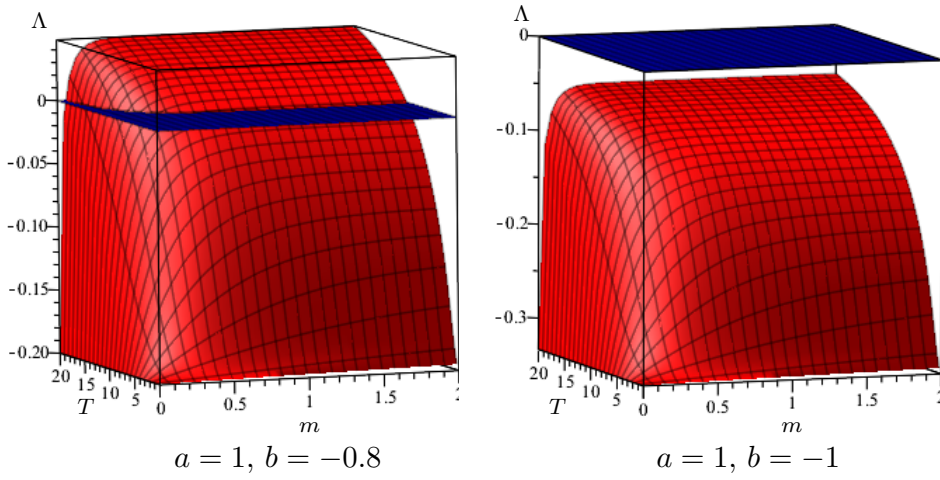
Fig. 9 If a = 1 then DIG occurs for -0.8 \leq b < -0.5 and does not occur for b \leq -1 .
