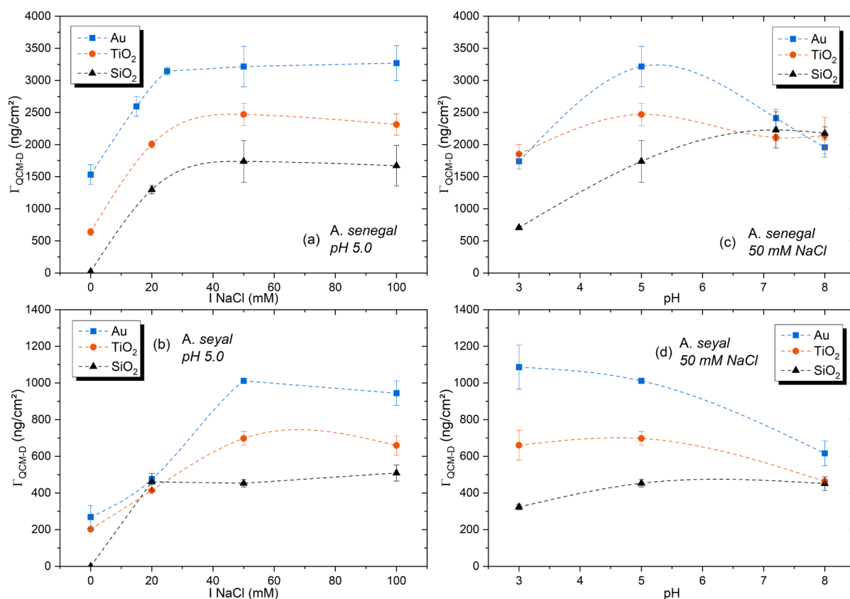
Figure 2. Adsorbed amount ( \Gamma_{\text{QCM-D}} ) onto Au (—■—), TiO 2 (—●—) and SiO 2 (—▲—) substrates at equilibrium state in function of NaCl ionic strength (a,b) at pH 5.0, and in function of pH at 50 mM NaCl (c,d) for A. senegal and A. seyal gums. Lines are here to guide the eyes.
