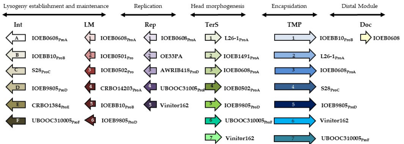
Figure 2. Scheme for the classification and rapid genotyping of oenophages. LM, lysogeny maintenance; Rep, replication-associated protein; TerS, small unit of the terminase; TMP, tape measure protein; Doc, toxin–antitoxin system. Representative phages containing the genes encoding the distinct proteins are indicated. Pro indicates that the phage is a prophage. Because some strains are poly-lysogens, the integrase type (A to F) is also indicated.
