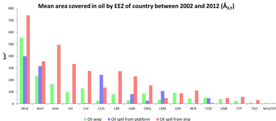
Figure 16. Mean area covered in oil by EEZs of countries ( \hat{A}_{X,Y} ) in the Gulf of Guinea between 2002 and 2012.
