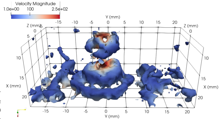
Figure 1: An isosurface of the Q criteria criteria in an impinging jet flow at Re = 1250 , color coded by the velocity magnitude (mm/s).
