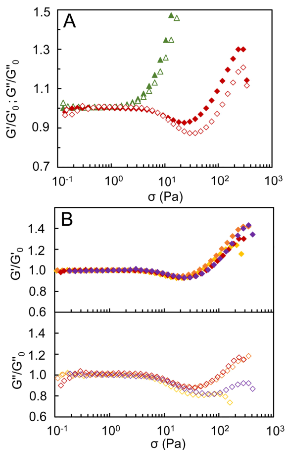
Fig. 3 (A) Stress sweep tests ( T = 30 °C, frequency f = 1 Hz) of an enzymatic milk gel (diamonds) and an acid milk gel (triangles): elastic modulus G' (full) and viscous modulus G'' (open) normalized by their value in the linear domains G'_0 and G''_0 , respectively, as a function of the stress amplitude ( \sigma ). Acid milk gel was prepared by adding glucono- \delta -lactone powder (1% w/w) to reconstituted skimmed milk and the stress sweep was initiated 20 h after glucono- \delta -lactone addition, i.e. at a final pH value of \approx 4.4 . (B) Stress sweep tests of an enzymatic milk gel at different frequencies: G' (full) and G'' (open) as a function of \sigma . Tested frequencies were f = 0.1 (yellow), 0.5 (orange), 1 (red) and 5 Hz (purple).
