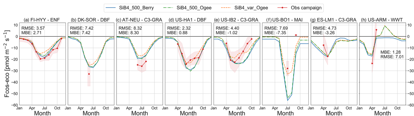
Figure 1. Comparison of ecosystem COS flux seasonal cycles of observations (red) with different SiB4 model runs: the original SiB4 with 500 pmol mol -1 COS and the original Berry soil model (SiB4_500_Berry, solid blue), a run with variable COS mole fractions and the Ogée soil model (SiB4_var_Ogee, dashed orange), and a run with 500 pmol mol -1 COS and the Ogée soil model (SiB4_500_Ogee, dash-dotted green). Monthly averages are shown with the 1 \sigma spread around the mean of observations. Negative values indicate uptake of COS by the ecosystem, while positive values indicate COS emissions. The model simulations are from the same year(s) in which observations were made. The MBE and RMSE (pmol m -2 s -1 ) are given for monthly average fluxes of the SiB4_var_Ogee run. Sites are presented from high to low latitude.
