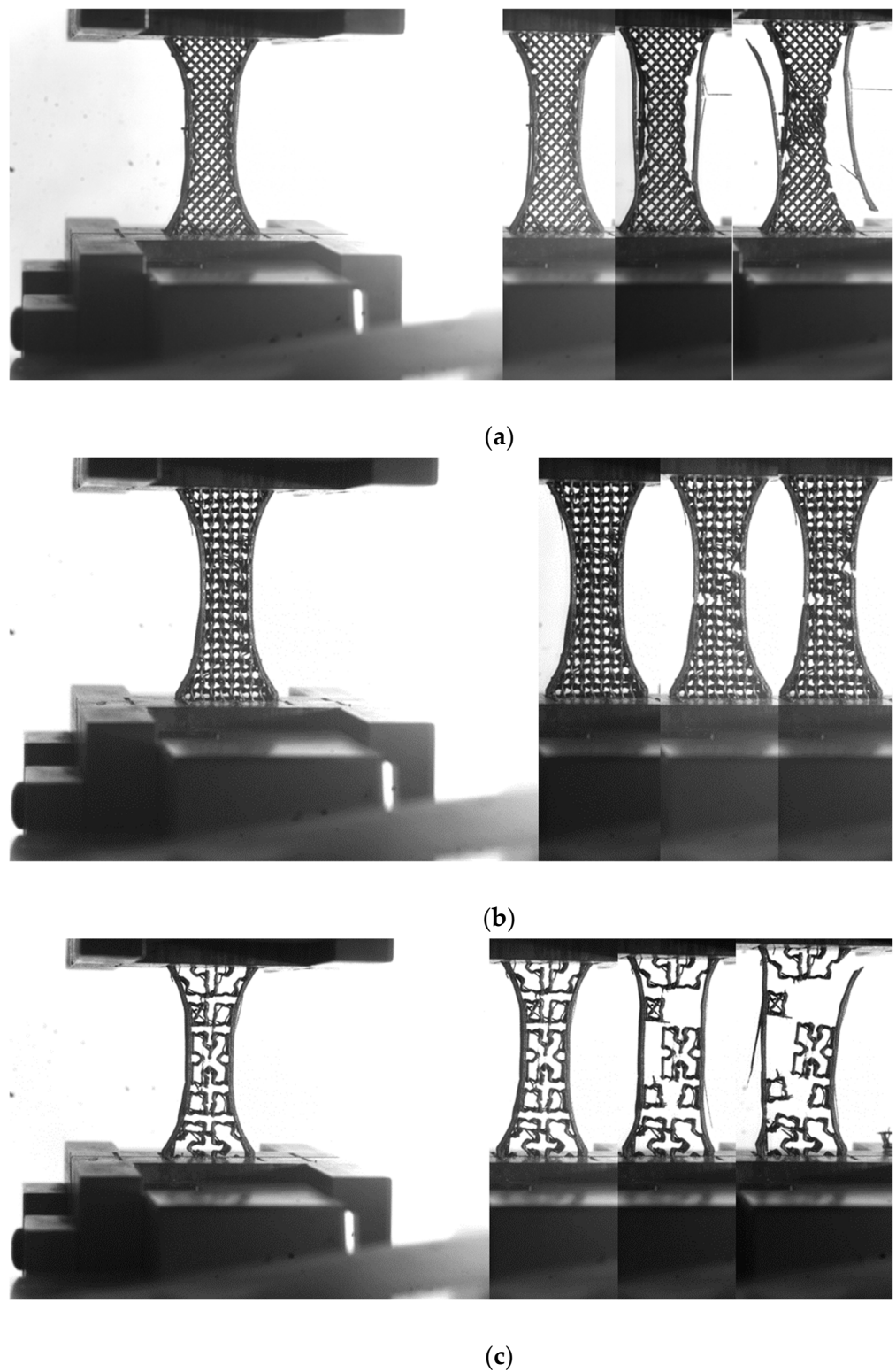
Figure 2. Deformation sequences of airy patterns (infill 25%): (a) zigzag, (b) gyroid, (c) cross.
