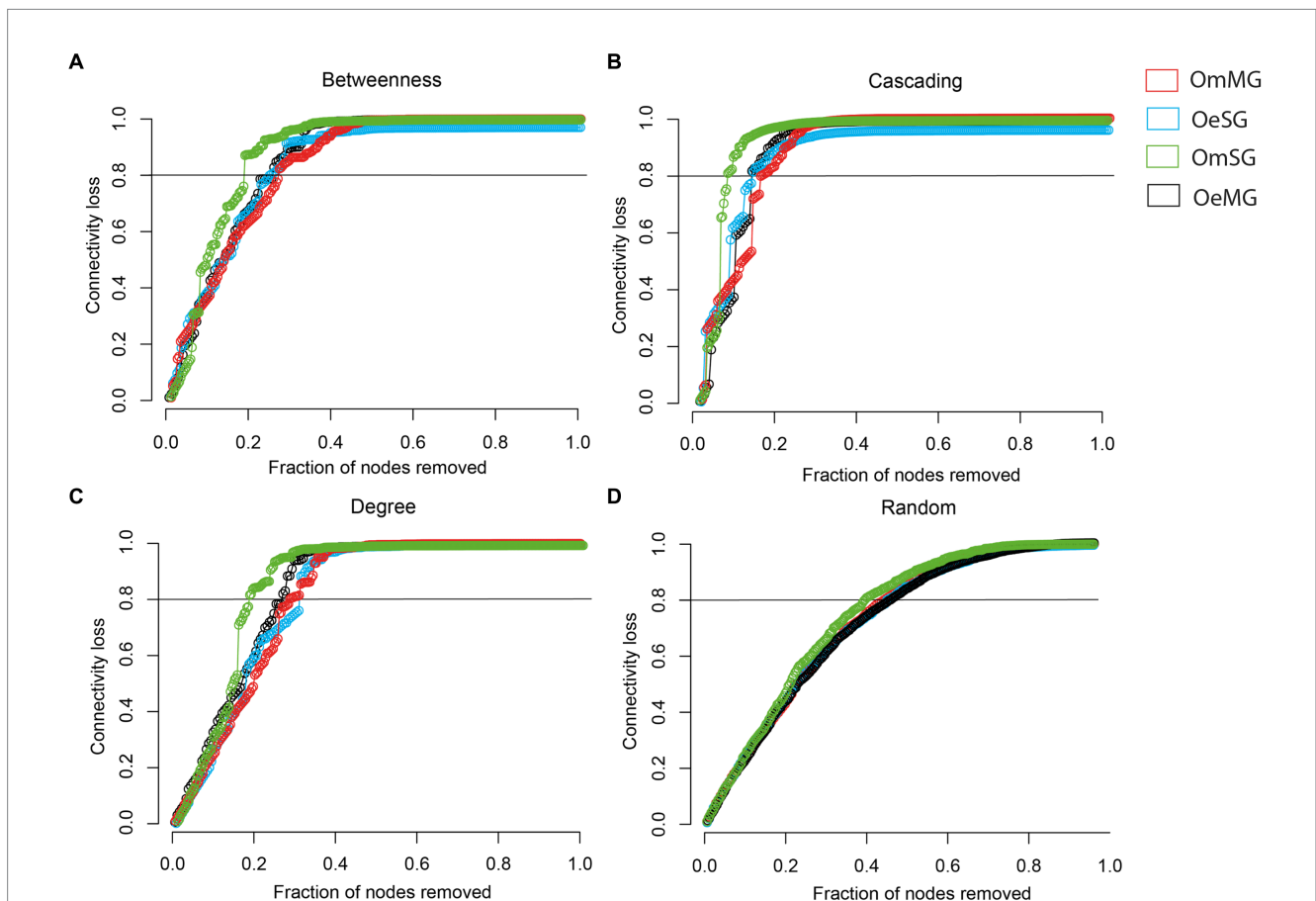
FIGURE 5 Robustness comparison of OeMG, OeSG, OmMG and OmSG networks. (A) Connectivity loss measured after directed attack, removing first the nodes with the highest betweenness centrality. (B) Connectivity loss measured after cascading effect, removing nodes with the highest betweenness centrality and recalculating the betweenness centrality value after each removal. (C) Connectivity loss measured after intentional attacks that target nodes with very high degree. (D) Connectivity loss measured after random removal of taxa in networks.
