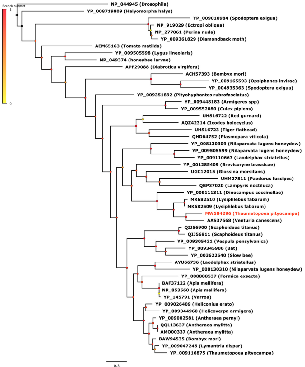
Fig. 2. Iflavirus phylogeny reconstructed by Maximum Likelihood method (midpoint rooted tree). For each virus, the name of the host is indicated in parenthesis. The newly identified iflaviruses of this study is written in red. Scale bar indicates number of amino acid changes per site and aLRT branch support values at each node are indicated by a color code.
