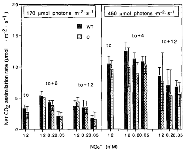
Fig. 8. The influence of N availability on net rate of CO 2 assimilation in leaves of WT and transgenic N. plumbaginifolia where the NR gene was constitutively expressed. Plants were grown at two levels of irradiance (170 and 450 \mu\text{mol photons} \cdot \text{m}^{-2} \cdot \text{s}^{-1} ) with a 16-h photoperiod, 23°C day, 18°C night at 12 mM NO 3 - for six weeks. Some of the plants were then transferred to either 0.2 or 0.05 mM N. Assimilation of CO 2 was measured 6 or 12 d after transfer to different levels of N nutrition for plants grown at 170 \mu\text{mol photons} \cdot \text{m}^{-2} \cdot \text{s}^{-1} and 4 and 12 d after transfer for plants grown at 450 \mu\text{mol photons} \cdot \text{m}^{-2} \cdot \text{s}^{-1}
