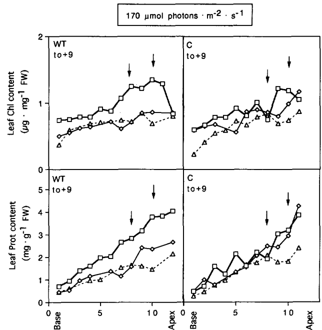
Fig. 1. The influence of nitrogen nutrition (12 mM \text{NO}_3^- \square – \square ; 0.2 \diamond – \diamond ; 0.05 \triangle – \triangle ) and leaf position on foliar chlorophyll and protein contents in low light-grown wild-type (WT) and transgenic (C) N. plumbaginifolia constitutively expressing NR. Plants were grown at 170 \mu\text{mol photons} \cdot \text{m}^{-2} \cdot \text{s}^{-1} with a 16-h photoperiod, 23° C day, 18° C night and 12 mM N for six weeks. Some of the plants were then transferred to either 0.2 or 0.05 mM N. Measurements were subsequently made 9 d after this transfer
