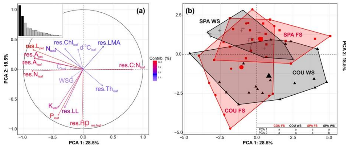
Figure 3 - Principal component analysis (PCA) on functional traits for the two sites for 70 trees. (a) Correlation circle of data with the histogram of inertia. (b) Individual factor map of data according to soil types and sites. In (a), the colour gradient indicates the contribution of each variable to the axis. See Table 3 for definitions of abbreviations. “Res” prefixes indicate residuals after removing the ontogenetical effect. In (b), significant differences in coordinates ( P < 0.05 ; ANOVA) between soil types and sites are indicated by letter according to the considered axis. Red: ferralitic soils; black: white-sand soils; COU: Counami; SPA: Sparouine.
