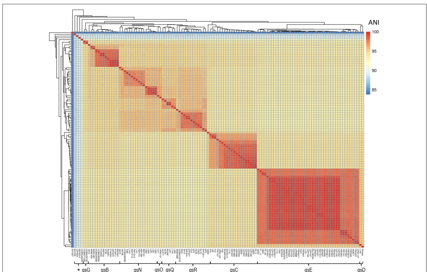
FIGURE 1 | Genomic diversity of the 121 Fabaceae symbiont selected for this study. Reference bacteria Sinorhizobium mellotii Sm1021, Rhizobium leguminosarum sv. trifolii WSM1689, Rhizobium leguminosarum sv. phaseoli Rlp4292 were also included in the comparison. Hierarchical clustering and heatmap were based on the Average Nucleotide Identity (ANI) values between each couple of the rhizobial genomes. Rlc genospecies classification (gs) has been based on an ANI threshold of 95%. Star gathered isolates phylogenetically distant to Rlc (88% < ANI < 92%), but included in the R. leguminosarum-etli clade. Additional informations are provided in the Supplementary Tables 1, 8 .
