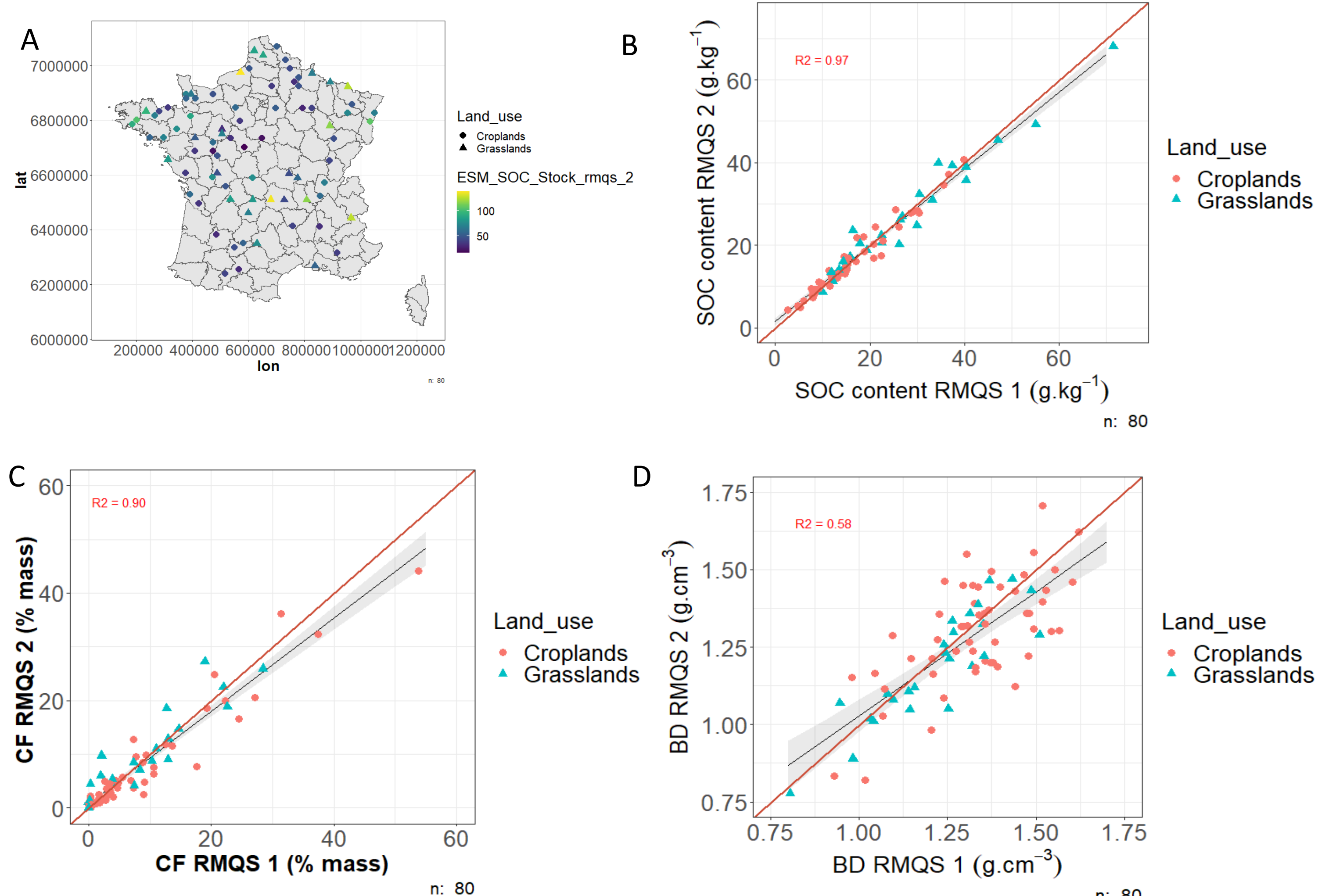
Figure 3. A) Spatial distribution of the sites. B) Soil organic carbon content, C) coarse fragments, and D) bulk density of RMQS 2 as a function of the values of RMQS 1 (black lines). Red lines are 1:1.
