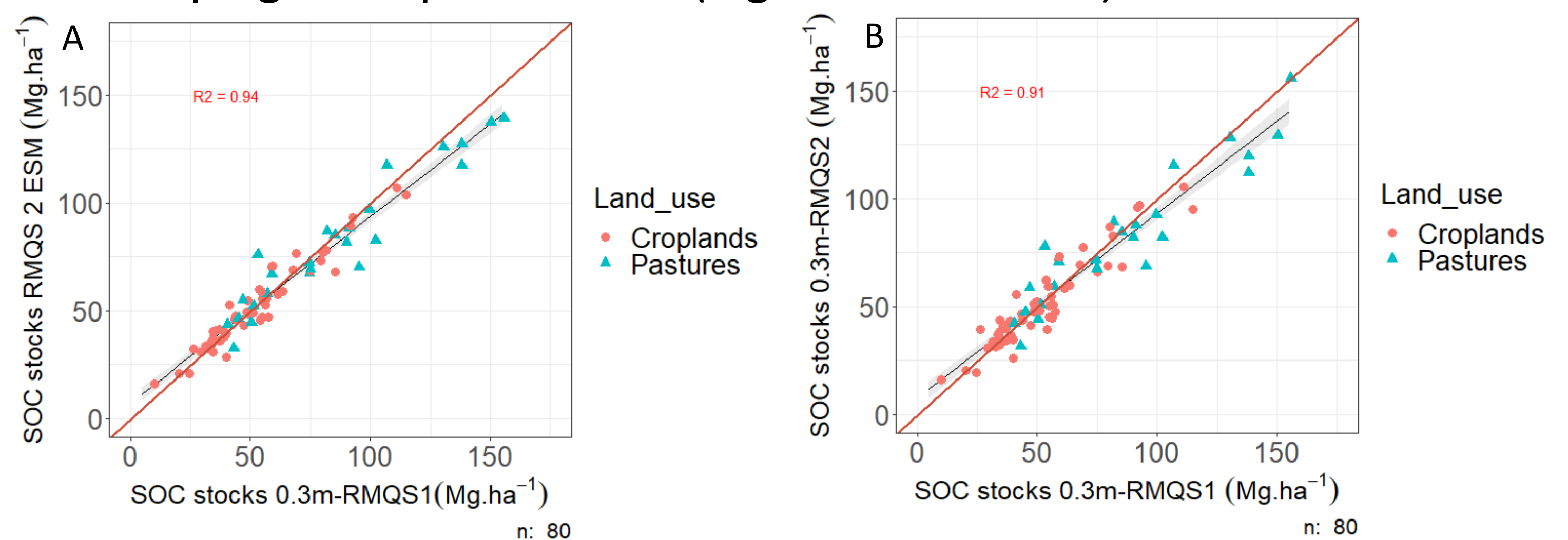
Figure 4. SOC stocks of RMQS 2 estimated based on A) ESM and B) FD as function of SOC stocks of RMQS 1 (black lines). Red lines are 1:1.
