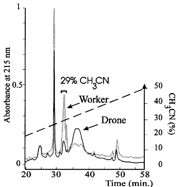
Fig. 1. Compared chromatographic profiles of worker and drone water-soluble antenna-specific protein. RPLC fractionation of water-soluble proteins from 100 antennae of workers or drones on a 2.1 × 100 mm Aquapore column in a 25 mM CH 3 COONH 4 , pH 6.8/CH 3 CN system. A linear gradient of 9.5–50% CH 3 CN was applied in 50 min at a flow rate of 200 µl/min. Dashed line indicates the CH 3 CN gradient.
