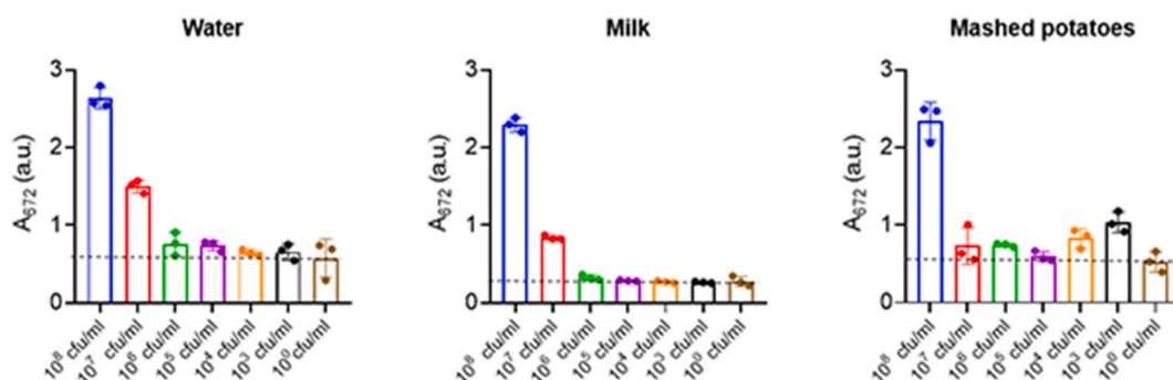
Fig. 5. Detection results for B. cytotoxicus spores in three different matrices using BAS6R@AuNPs aptasensor. Quantitative evaluation was performed by measuring absorption at 672 nm. Individual data points ( n = 3 independent experiments) are shown; error bars represent means \pm SD.
