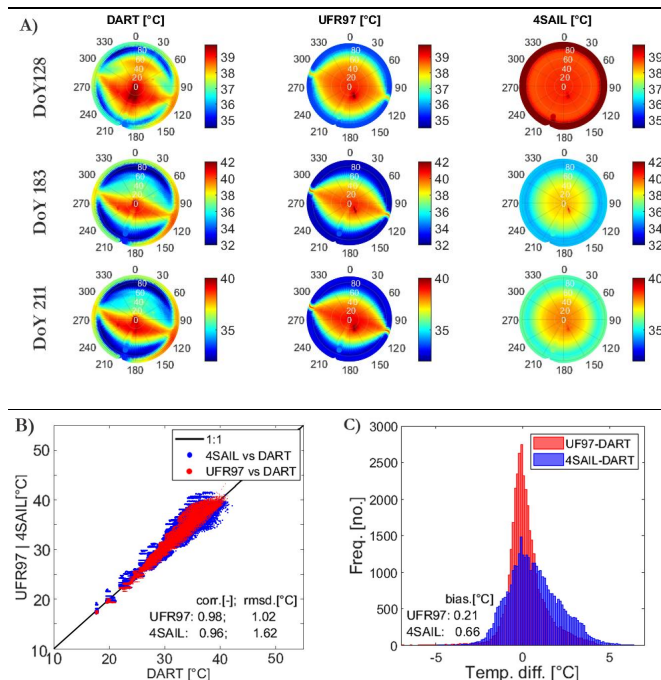
Figure 4: Inter-comparison of the UFR97 (and 4SAIL) temperatures to those simulated by the DART 3-D radiative transfer model. A) noon polar plots depicting the simulated angular temperatures; presented separately for the 3 selected
