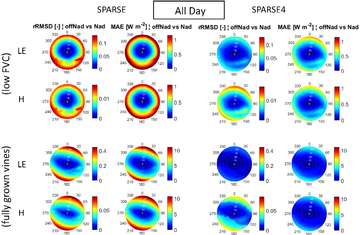
Figure 7: LE and H polar plots of oblique-vs-nadir rRMSD and MAE for the growth period – i.e., periods with low vegetation cover and with fully grown vines [noon and all-day]
