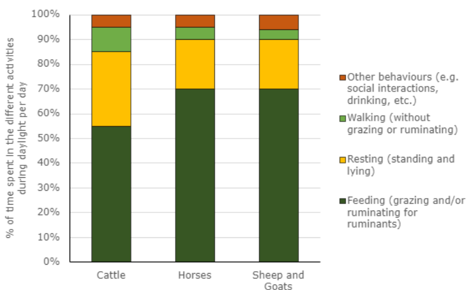
Figure 1: Summary of the estimated time-budget behavioural activity on pasture during daylight for cattle, horses, sheep and goats (Ishiwata et al., 2008; Maisonpierre et al., 2019; Neave et al., 2021; Pokorná et al., 2013; Waring, 2003).
