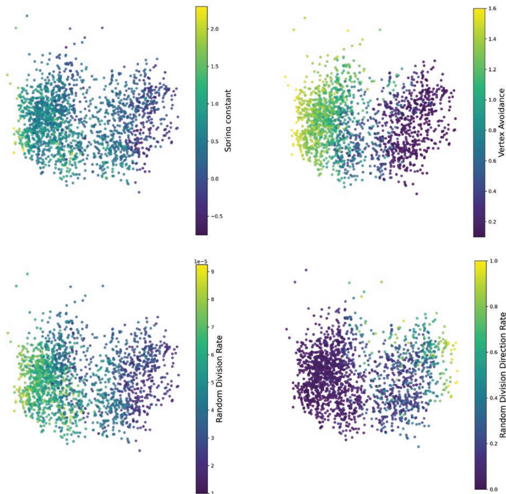
Figure 8. Visualizing simulation parameters using Diff2Dist. Each plot shows one point for each morphological graph in our Arabidopsis data set. Points are placed in 2D using Isomap, exactly as in Fig. 7. Points are coloured according to the parameter values of the nearest simulation-derived graphs, where means in the sense of our trained distance metric.
