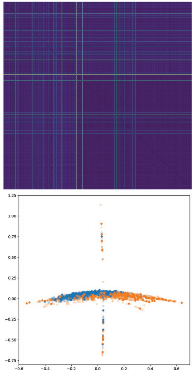
Figure 5. As in Fig. 4, but for method 2 (weighted norm GDD on graphs with fixed Gaussian kernel edge weights.). This distance matrix and embedding have the same flaws as those in Fig. 4.
