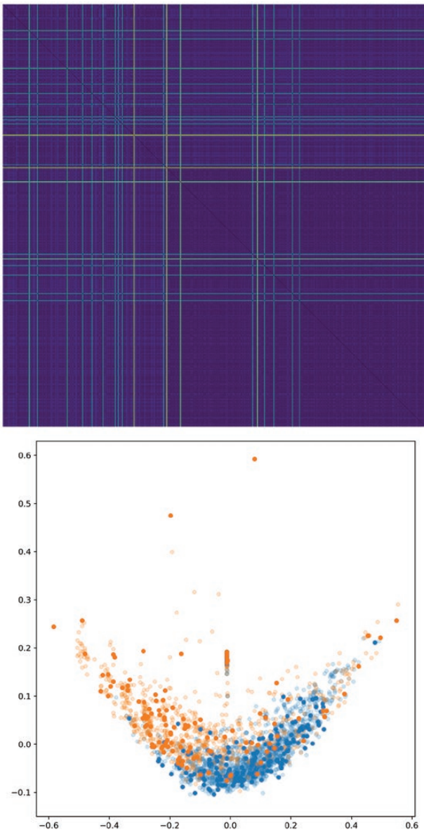
Figure 4. Top: distance matrix for morphological graphs, generated with method 1 (GDD on unweighted graphs). Bottom: Isomap embedding of this distance matrix, which ensures that points with small distance are placed near each other. Blue points represent the wild type, and orange points represent the mutant. Transparent points represent training set graphs; solid points represent those from the test set. We see that naive GDD leads to an embedding where the two categories of graph overlap, indicating that GDD by itself is not capturing the distinction between these two classes of graph.
