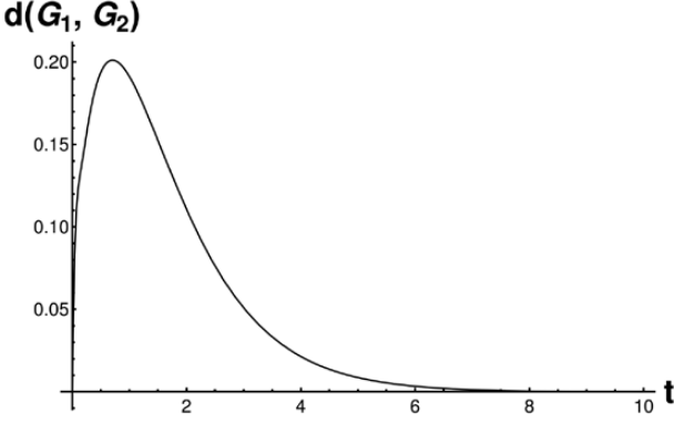
Figure 2. This figure shows the result of evaluating the norm in Equation (1) with eigenvalues of two random graphs on 32 nodes, for varying values of t . This demonstrates why we take the diffusion distance to be the peak of this norm; since at early and late times the difference between the eigenvalues of the two diffusion kernels vanishes.
