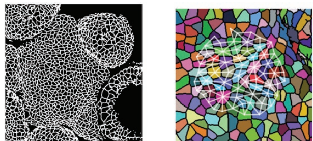
Figure 3. Left: an image of the SAM of a mutant Arabidopsis specimen. The original 3D confocal microscope image is here represented as a 2D skeleton. Right: a zoomed-in view of the same specimen, with separate cells false-coloured and an example extracted cell neighbourhood graph overlaid.
