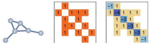
Figure 1. From left to right: a small graph, its adjacency matrix and its graph Laplacian.
