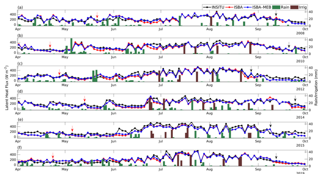
Figure 5. The 2-days average daytime series of the in situ latent heat flux ( LE ) (in black) with those estimated by ISBA (in red) and ISBA-MEB (in blue). Panels (a–f) represent the plots for 2008, 2010, 2012, 2014, 2015, and 2019, respectively. The red and black arrows signify the planting and the harvest days, respectively.
