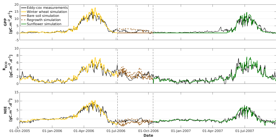
Figure 3. Temporal evolutions of the gross primary productivity (GPP), the ecosystem respiration ( R_{ECO} ), and the net ecosystem exchange (NEE). Winter wheat, bare soil, regrowth, and sunflower periods are displayed in yellow, brown, dashed brown, and green respectively.
