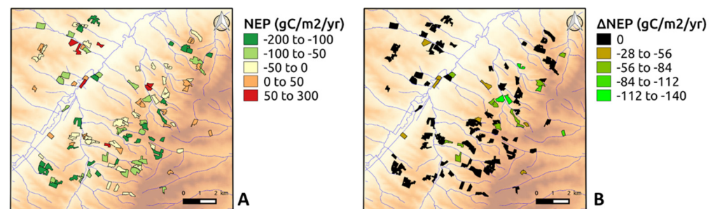
Figure 4. Spatial distribution of the net ecosystem productivity (NEP) simulated over 111 fields without taking regrowth events into account (A), and the differences in the scenario where regrowth events are considered (B).
