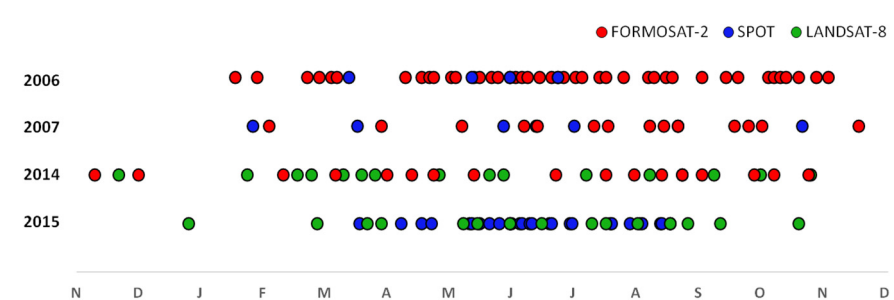
Figure 2. Timeline of satellite images used in this study.
