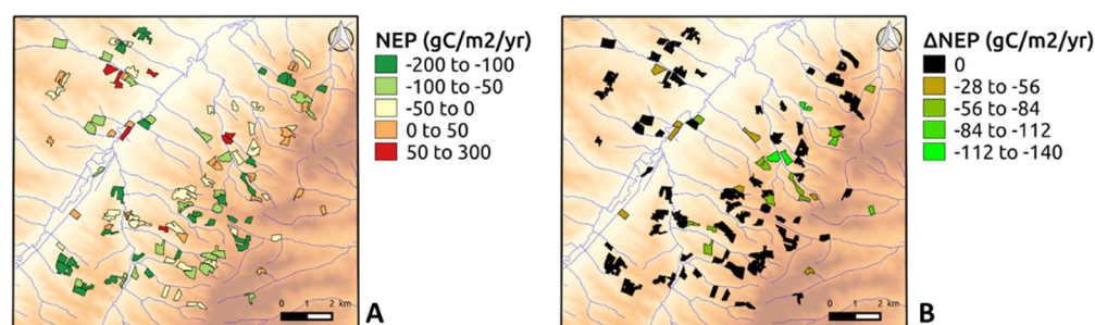
Figure 4. Spatial distribution of the net ecosystem productivity (NEP) simulated over 111 fields without taking regrowth events into account (A), and the differences in the scenario where regrowth events are considered (B).
