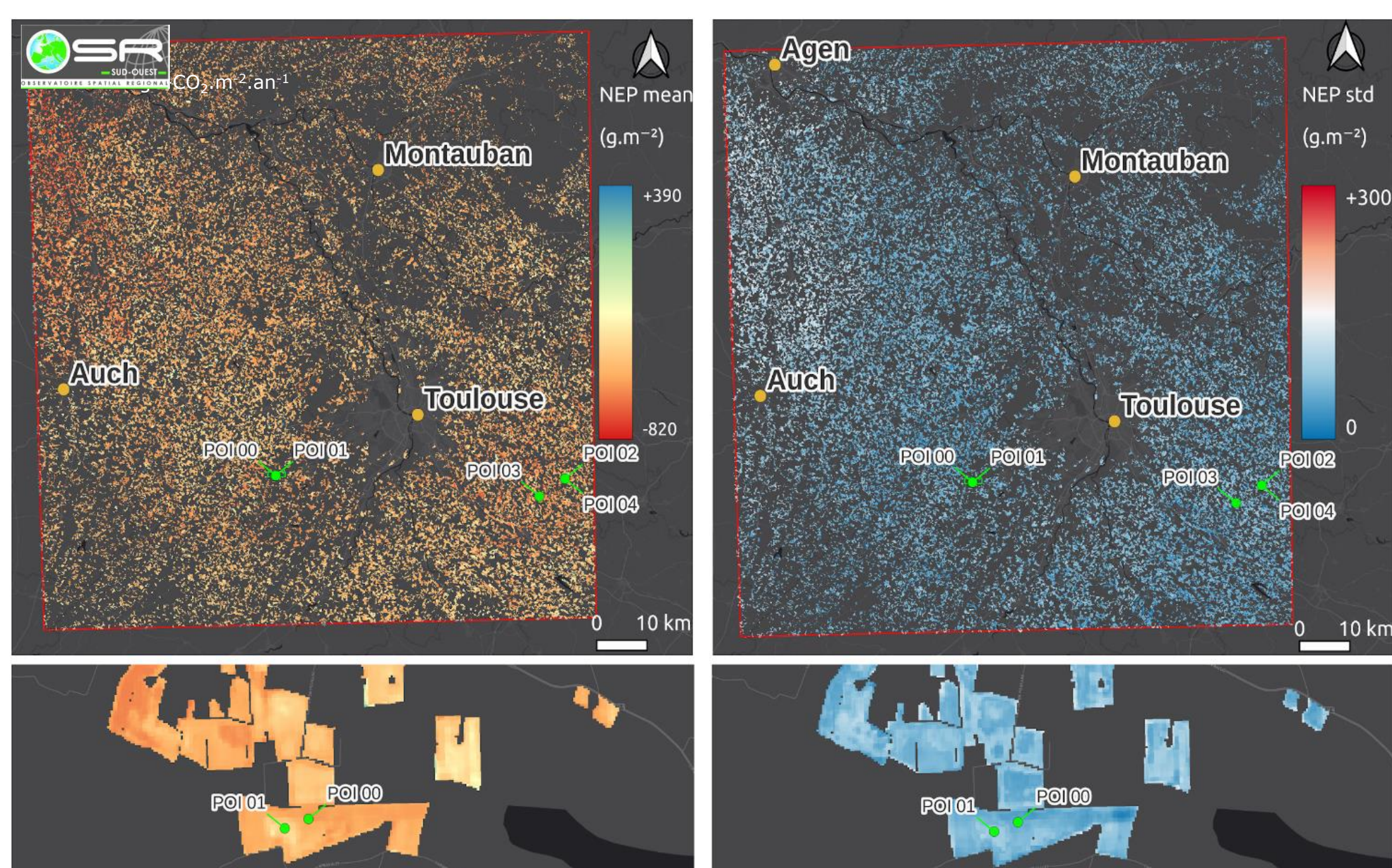
Example of net annual CO 2 fluxes at 10m resolution for straw cereals in 2017 (left average and right uncertainty) in South West France
