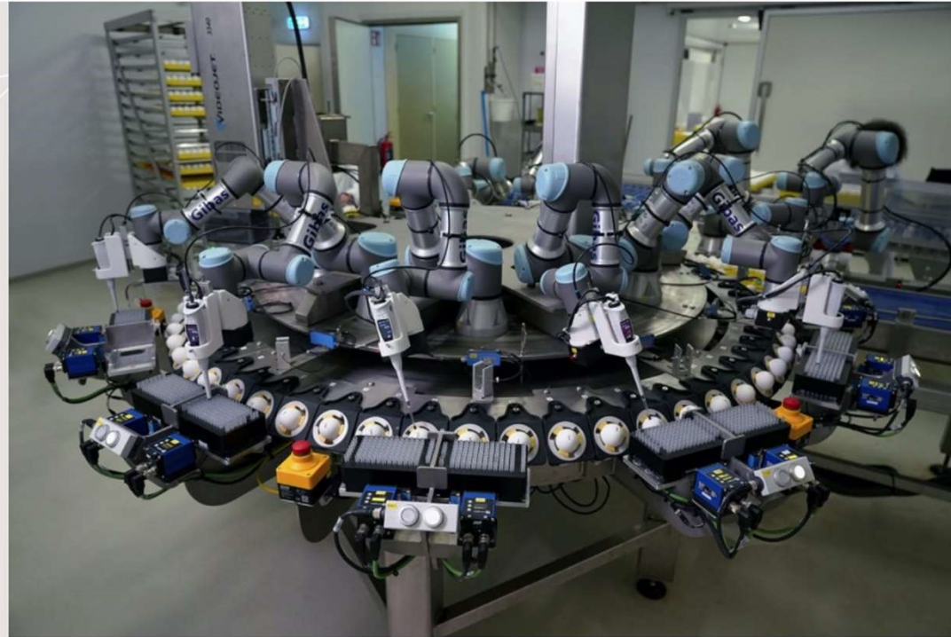
The SELEGGT process is a way to prevent chick culling. The scientific approach of endocrinological (hormone-based) gender identification in the hatching egg has been automated in the SELEGGT process and is already in use today.
