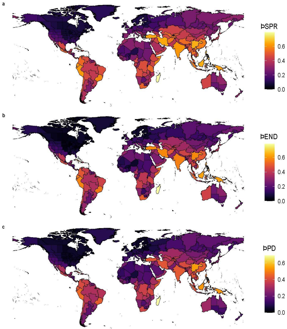
Extended Data Figure 2 | Distribution of plant diversity ( \mathfrak{P}SPR , \mathfrak{P}END , \mathfrak{P}PD ) that is under threat | (a) polygons with the highest proportion of threatened species ( \mathfrak{P}SPR ). (b) polygons with the highest proportion of threatened endemics ( \mathfrak{P}END ) compared to the total number of species in that polygon. (c) polygons with the highest proportion of threatened phylogenetic diversity ( \mathfrak{P}PD ).
