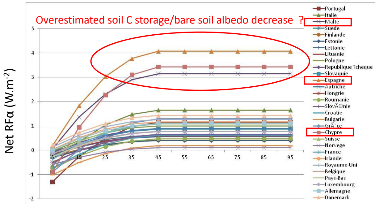
Adapted from Tribouillois et al (2018) and considering Corg max similar to Romanian soils
