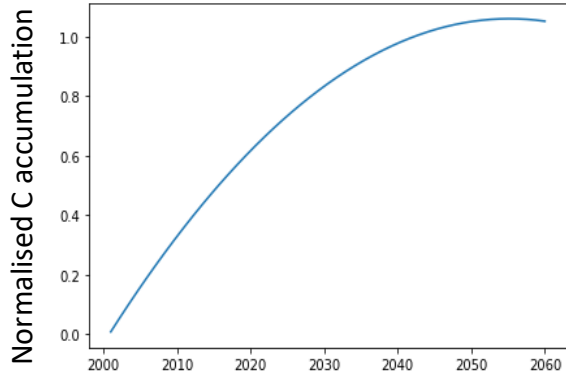
Adapted from Tribouillois et al (2018) and considering Corg max similar to Romanian soils
