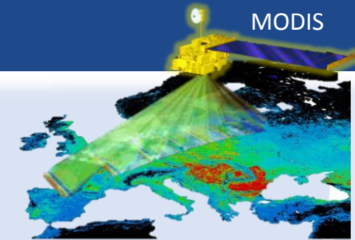
Surface albedo dynamics
