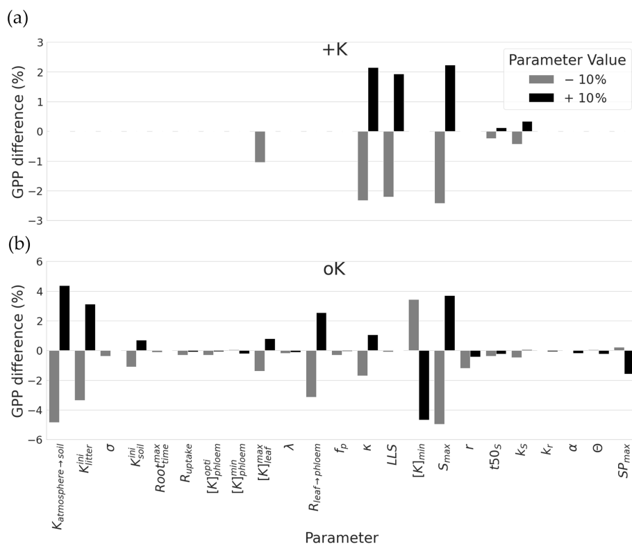
Figure 7. Sensitivity of GPP cumulated over a rotation to a \pm 10\% change in parameters related to soil availability, diffusion resistances, and response of leaves development to K. For each parameter, the sensitivity analysis was performed for the two contrasting K supply regimes (+K and oK). Note differences on the y axes scales for the sake of clarity.
