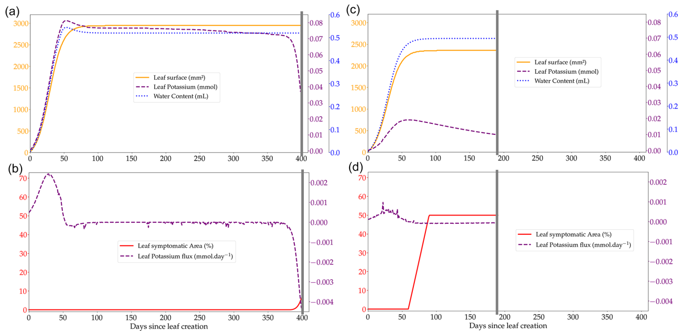
Figure 2. Outputs of the leaf cohort expansion model over the course of the lifespan of a single leaf from a cohort (produced on day 504 of the rotation at the Itatinga site) in two contrasted K availabilities, +K (a, b) and oK (c, d); leaf water content, leaf K, and leaf surface at the individual leaf scale (a, c); total flux of K at the leaf scale showing the transition from K sink (positive flux to the leaf) to K source (negative flux from the leaf) (b, d). Small negative K fluxes (corresponding to a loss of K from the leaf) during the leaf's existence are K foliar leaching fluxes during precipitation events. The grey line represents the fall of the leaf cohort. The quantity of K that is in the leaf at the moment of leaf fall is added to the K litter pool.
