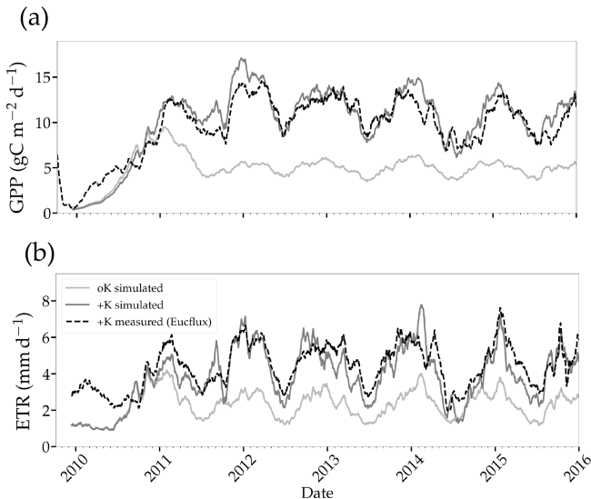
Figure 6. Simulated and measured daily gross primary productivity (a) and evapotranspiration (b) fluxes simulated in two stands with contrasted fertilisation regimes. The measurements were performed continuously using the eddy covariance method at the EUCFLUX site (a +K stand, fully fertilised). A rolling average of 30 d was applied to the observed and simulated time series for the sake of clarity.
