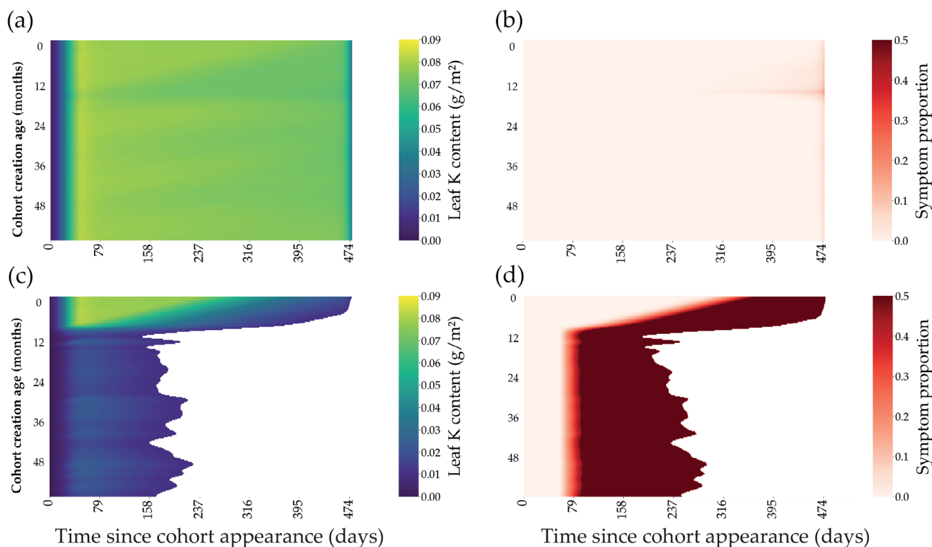
Figure 4. Outputs of the leaf cohort model in two contrasted K fertilisation regimes. The K content present in each individual leaf of the cohort is represented through the lifespan of a cohort ( x axis) for the different cohort created along the first 60 months of the rotation (a, c). The symptom area proportion for each leaf of the cohort is also represented (b, d). Top subplots (a, b) were simulated in +K conditions, while bottom subplots were oK simulations (c, d).
