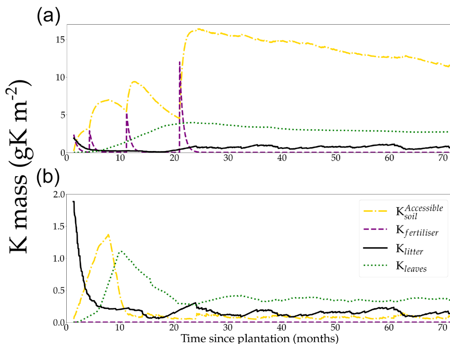
Figure 3. Simulated stocks of K in the soil, litter, fertiliser, and canopy compartments in a non-K-limited (+K) stand (a) and in the same K-limited (oK) stand (b). Note differences of the y axis scales for better visualisation.
