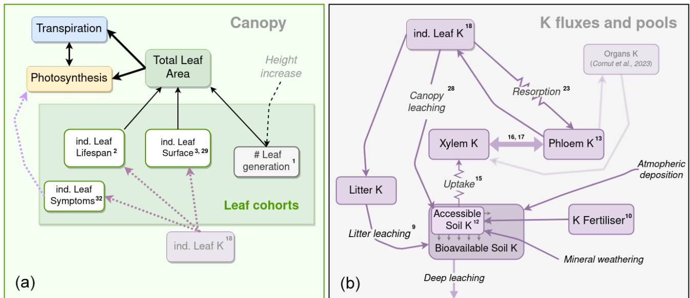
Figure 1. Schematic representation of the soil and plant components of the K cycle, and their links with the leaf cohort model and other sub-models. On the left is a schematic representation of the canopy leaf cohort sub-model. Black arrows represent a functional link a variable has with another variable or process. Dashed lines represent an influence of one process (black), pool (purple), or state (light purple) over a process or pool. On the right a schematic representation of the K flux and pool sub-model. Purple boxes are K state variables, and purple arrows are K fluxes. K fluxes simulated with a simple Ohm's law form are represented with resistance symbols. The numbers in exponential form correspond to the numbers of the equation in the text. The K pools of other organs (woody and roots) and their link to the K circulation model are semi-transparent, since they are described in the companion paper (Cornut et al., 2023).
