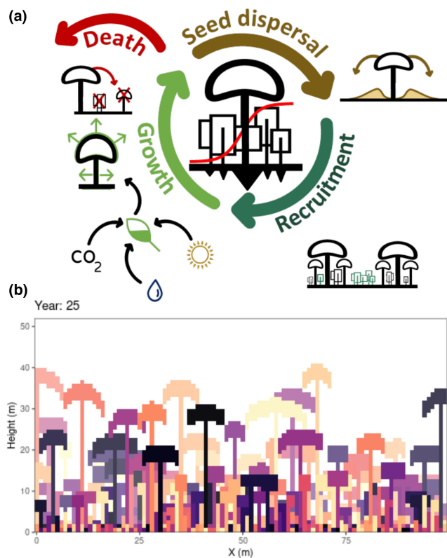
FIGURE 1 TROLL forest simulator. (a) TROLL is a spatially explicit and individual-based forest model, which simulates carbon assimilation and allocation (light green), trunk and crown growth (light green), seed dispersal (brown) and tree deaths (red) and recruitments (dark green). (b) Output from a TROLL simulation using the autogif function in the rcontroll package. The image shows a vertical cut in the forest structure along the x-axis (in metres) with individual tree height (metres) on the y-axis. The tree colours indicate the identity of the species and can be changed using the ggplot2 grammar. The figure shows the forest structure after 625 years of a successional trajectory starting from bare ground, which can be seen dynamically over 200 years at https://raw.githubusercontent.com/sylvainschmitt/rcontroll/main/inst/figures/troll.gif .
