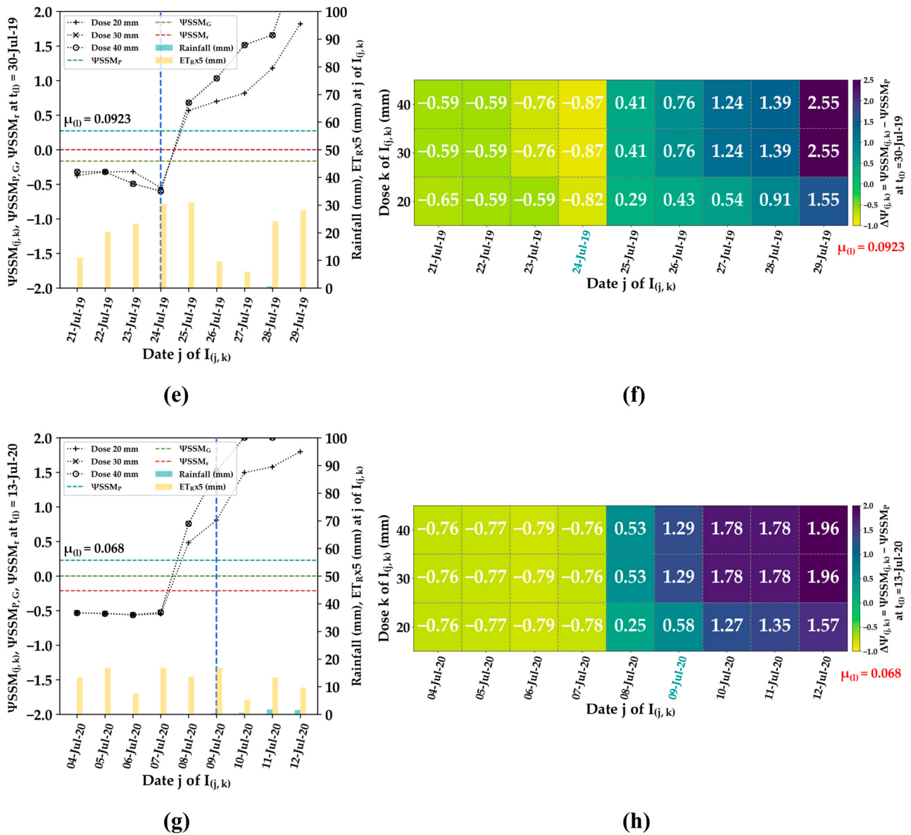
Figure 6. Irrigation detection using the evening SAR acquisition over P1 for t_l = 6 August 2017 (a,b), P2 for t_l = 30 August 2018 (c,d), P3 for t_l = 30 July 2019 (e,f) and the morning SAR acquisition over P4 for t_l = 13 July 2020 (g,h). In (a,c,e,g), the calculated \Psi\text{SSM}_{R(i,k)} (rate of change of \text{SSM}_{R(i,k)} ) between t_l and t_{(i)} as a function of k of the injected irrigation I_{(j,k)} is represented by the black lines for k = 20, 30 , and 40 mm. The vertical dash lines in dark blue represent the real irrigation dates ( d_{Re} ). The light blue, green, and red horizontal dash lines represent the \Psi\text{SSM}_P , \Psi\text{SSM}_G , and \Psi\text{SSM}_T , respectively. In (b,d,f,h), the difference \Delta\Psi_{(i,k)} = \Psi\text{SSM}_{R(i,k)} - \Psi\text{SSM}_P is represented by the white values in the matrix for each I_{(j,k)} . The date j in blue indicates the d_{Re} and \mu_0 indicates the value of the error on \Psi\text{SSM}_P .
