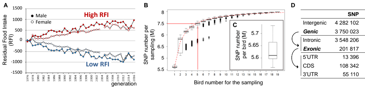
Figure 6. Characteristics of the SNP found within the genome of the high RFI and low RFI lines. A. Line responses to selection for RFI, B. Estimation of the number of SNP to be detected by resampling 1000 times combinations of 1 to 19 birds, C. Distribution of the number of SNP detected per bird, D. Distribution of the detected SNP depending on the genome annotation.
