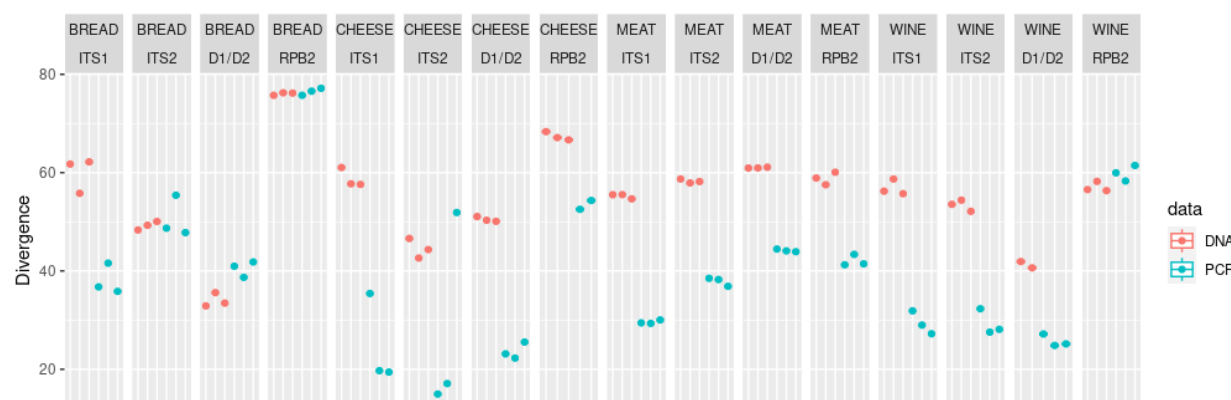
Figure 7 - Divergence at species level for each tested barcode marker and mock community. DNA mock communities are colored in red and PCR mock communities are colored in blue.
