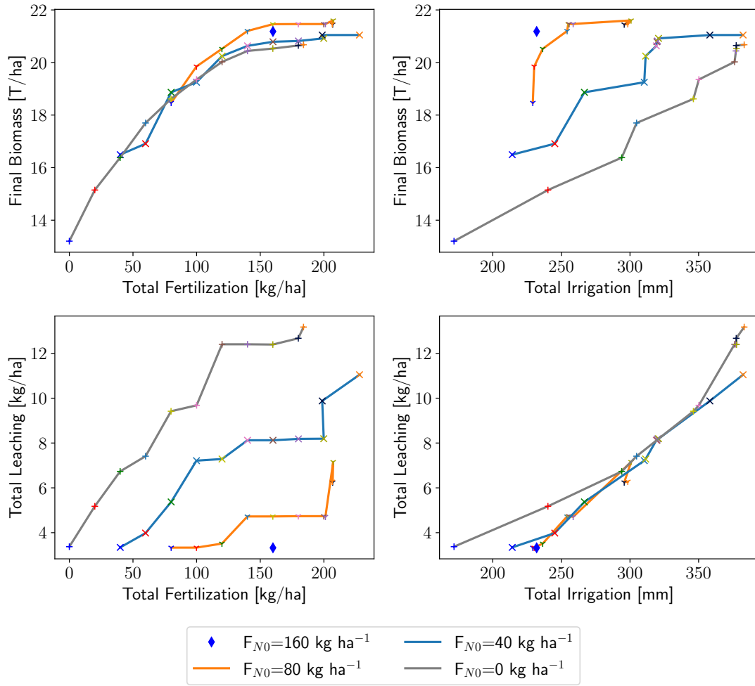
Figure 7: Final crop biomass and total leaching as a function of total fertilization \mathcal{P} = F_{N0} + \int_{t_0}^{t_f} F_N(t) dt and irrigation. Values from the simulation model are shown for 3 different initial fertilizations F_{N0} for the standard experiment. Each color of markers correspond to a value of \bar{F} , the upper bound on the total N added through irrigation, and for example, red markers are values associated with \bar{F} = 20 kg ha -1 . For comparison, results are shown (blue diamond) for the case of an initial fertilization of 160 kg ha -1 and irrigation without nitrogen, i.e. the solution for \bar{F} = 0 .
