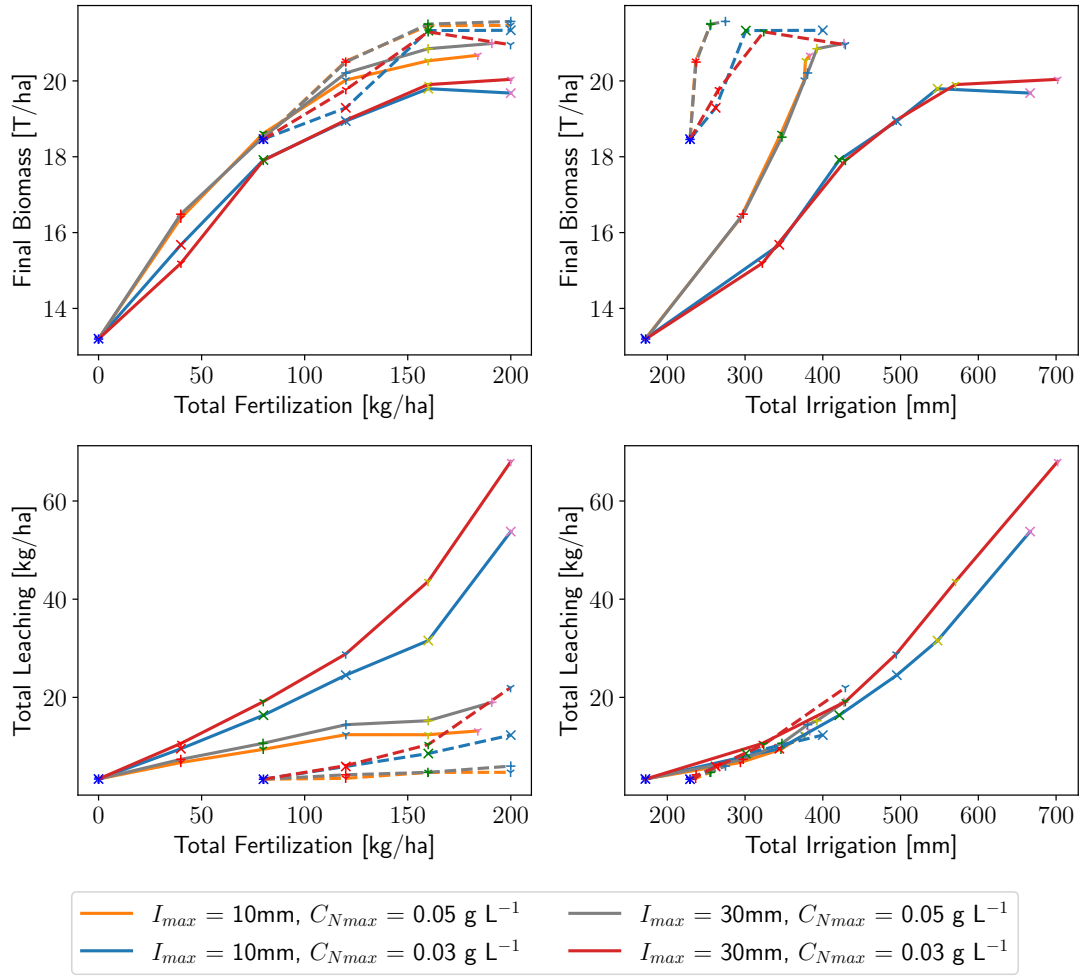
Figure 8: Impact of control bounds on final crop biomass and total leaching, as a function of total fertilization P = F_{N0} + \int_0^f F_N(t) dt and irrigation. Values from the simulation model are shown for F_{N0} = 0 (solid lines) and for F_{N0} = 80 \text{ kg ha}^{-1} (dashed lines) for different values of the control bounds ( I_{max} and C_{Nmax} ). Each color of markers correspond to a different value of \bar{F} , the upper bound on the total N added through irrigation.
