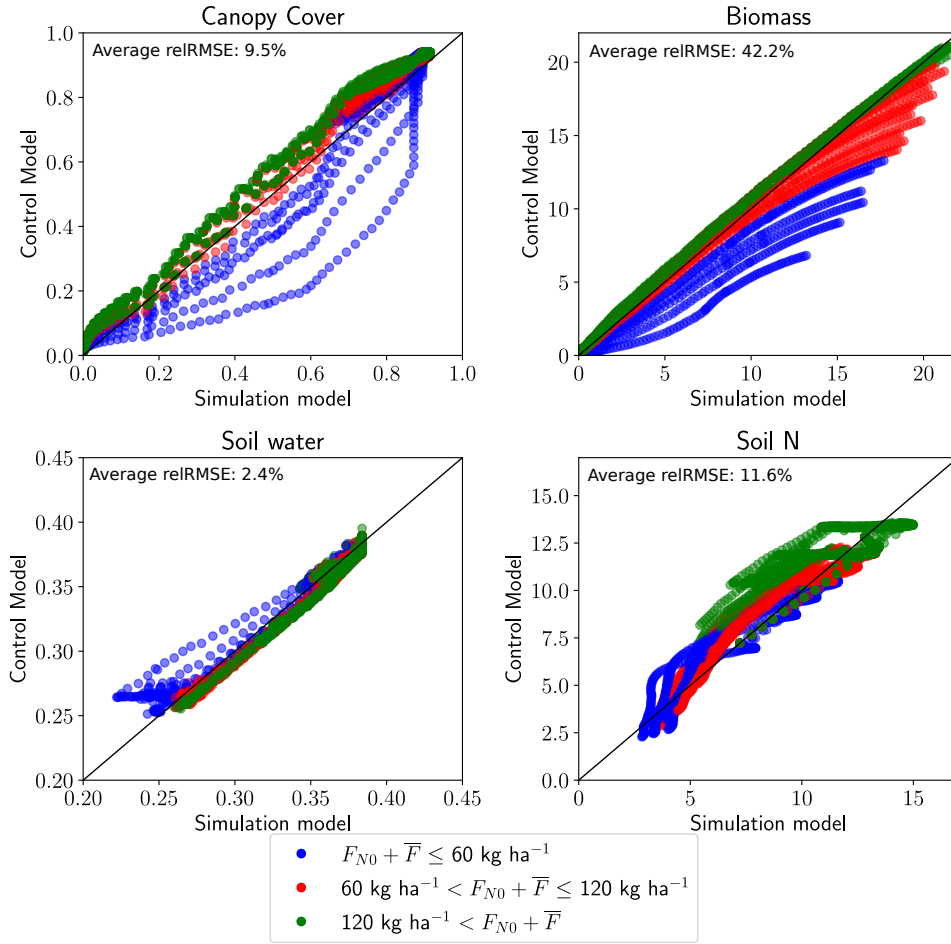
Figure 3: Values of control model variables plotted against values of simulation model for all simulations of the standard experiment. Colors indicate the total fertilization \bar{F} which is the sum of initial input F_{N0} and input through irrigation \bar{F} .
